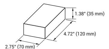
Driver Dimensions
