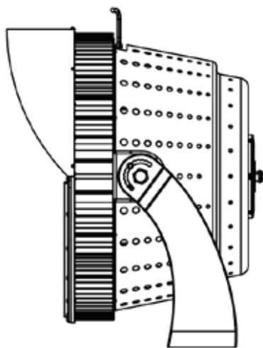
Side EPA: 0.260m 2 | 2.79ft 2
