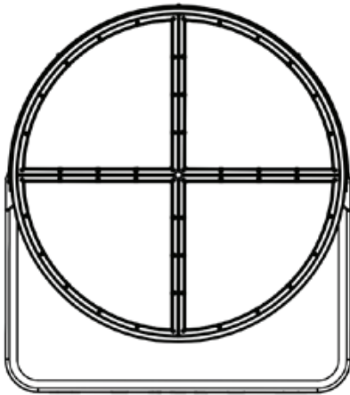
Front EPA: 0.187m 2 | 2.01ft 2
