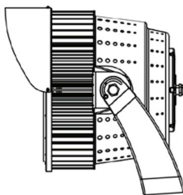
Side EPA: 0.108\text{m}^2 | 1.16\text{ft}^2
