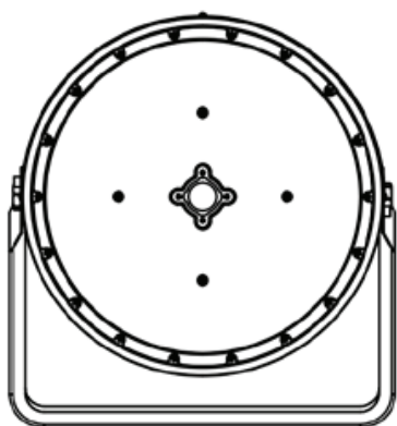
Front EPA: 0.116\text{m}^2 | 1.25\text{ft}^2
