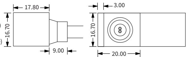
Side Entry Connector YYZ-MIC-SEC-01 (Single Feed-Right Side) YYZ-MIC-SEC-02 (Single Feed-Left Side) YYZ-MIC-SEC-03 (Double Feed-Both Side)
