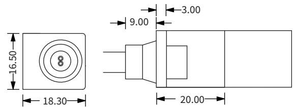
Direct Entry Connector YYZ-MIC-DEC-01 (Single Feed-Right Side) YYZ-MIC-DEC-02 (Single Feed-Left Side) YYZ-MIC-DEC-03 (Double Feed-Both Side)
