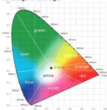
Wavelength of Color Light
